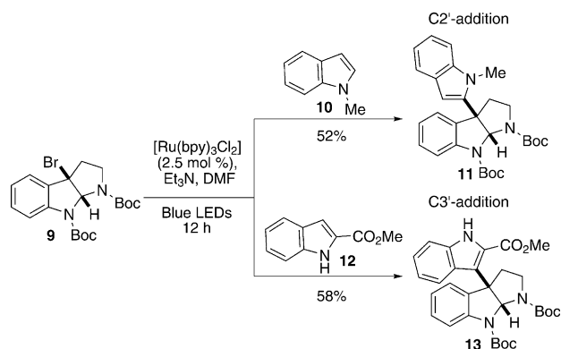
Scheme 2. Visible-light-mediated coupling of bromopyrroloindoline 9 with indoles enables selective access to both C2'- and C3'-substituted bisindoles. Boc = tert -butoxycarbonyl.
