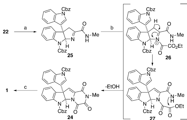
Scheme 4. a) NBS, CH 2 Cl 2 , DBU, 23 °C, 99%; b) ClCOCO 2 Et, Et 3 N, 150 °C, microwave, 0.5 h, 76 % (90 % conversion, two cycles); c) BCl 3 , CH 2 Cl 2 , -78 °C to 23 °C, 12 h, 80 %. DBU = 1,8-diazabicyclo-[5.4.0]undec-7-ene.
