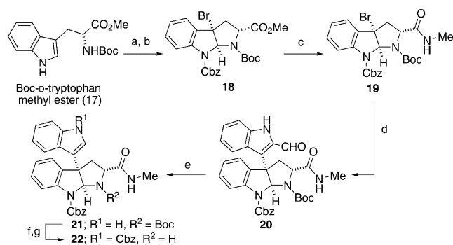
Scheme 3. a) CbzCl, NaOH, Bu 4 NHSO 4 , CH 2 Cl 2 , 12 h; b) NBS, PPTS, CH 2 Cl 2 , 23 °C, 12 h, 91% (two steps); c) MeNH 2 , THF, 23 °C, 3 d, 87%; d) [Ru(bpy) 3 Cl 2 ] (1.0 mol %), Bu 3 N (2 equiv), 15 (5 equiv), DMF, blue LEDs, 12 h, 82%; e) [Rh(Ph 3 P) 3 Cl] (1 equiv), xylenes, 140 °C, 12 h, 86% or [Rh(CO)(Ph 3 P) 3 Cl] (20 mol %), dppp (44 mol %), DPPA (2 equiv), xylenes, 140 °C, 85%; f) CbzCl, NaOH, Bu 4 NHSO 4 , CH 2 Cl 2 , 12 h, 98%; g) TMSI, CH 3 CN, 0 °C, 1 h, 91%. Cbz = benzyloxycarbonyl; DMF = N,N' -dimethylformamide; DPPA = diphenylphosphoryl azide; dppp = 1,3-bis(diphenylphosphino)propane; LED = light-emitting diode; NBS = N -bromosuccinimide; PPTS = pyridinium p -toluenesulfonate; THF = tetrahydrofuran; TMS = trimethylsilyl.
